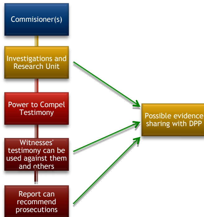
Figure 3: Truth Commission and Prosecutions
